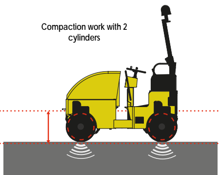
Vibrating drums
